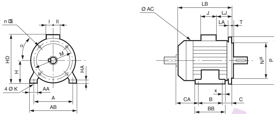
Main Dimensions
