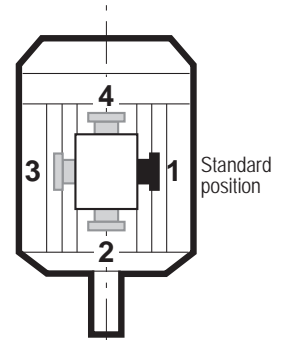
Positions of the cable gland relative to the motor shaft end
