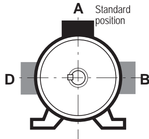
Positions of the terminal box relative to the motor shaft end
