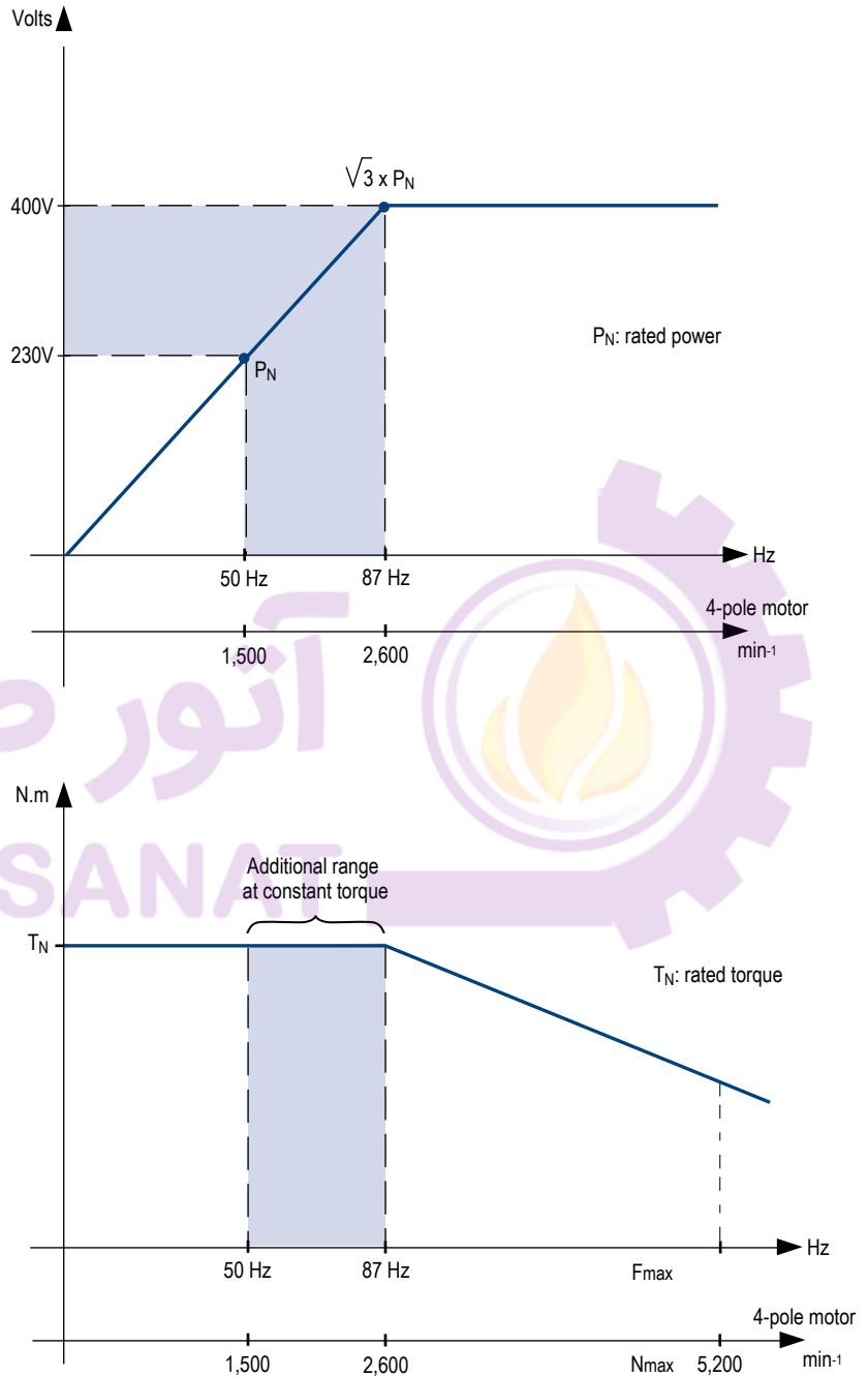
Characteristics of motors on drives 230 V Δ connection 400 V 50 Hz supply
