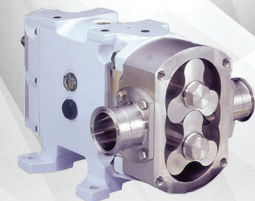
Lobe Pump
