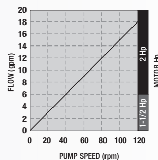
EP4029 Performance
