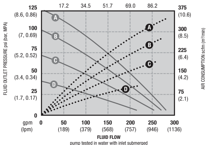
Husky 3300 Performance
