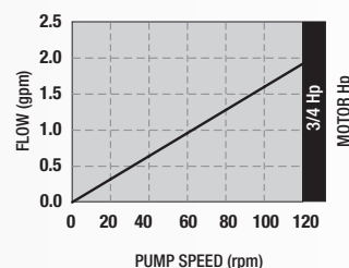
EP2013 Performance
