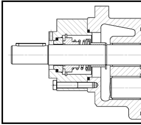
Fig. 6: Mechanical seal
