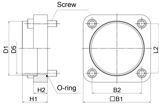
Weld-on flange
