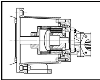
Fig. 7: Magnetic coupling
