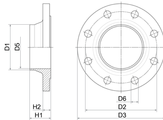
Weld-on flange
