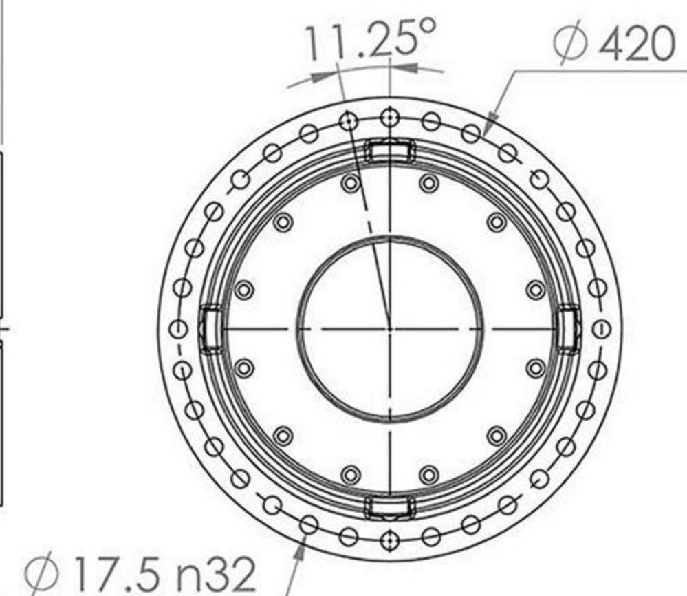
Output Flange Dimensions
