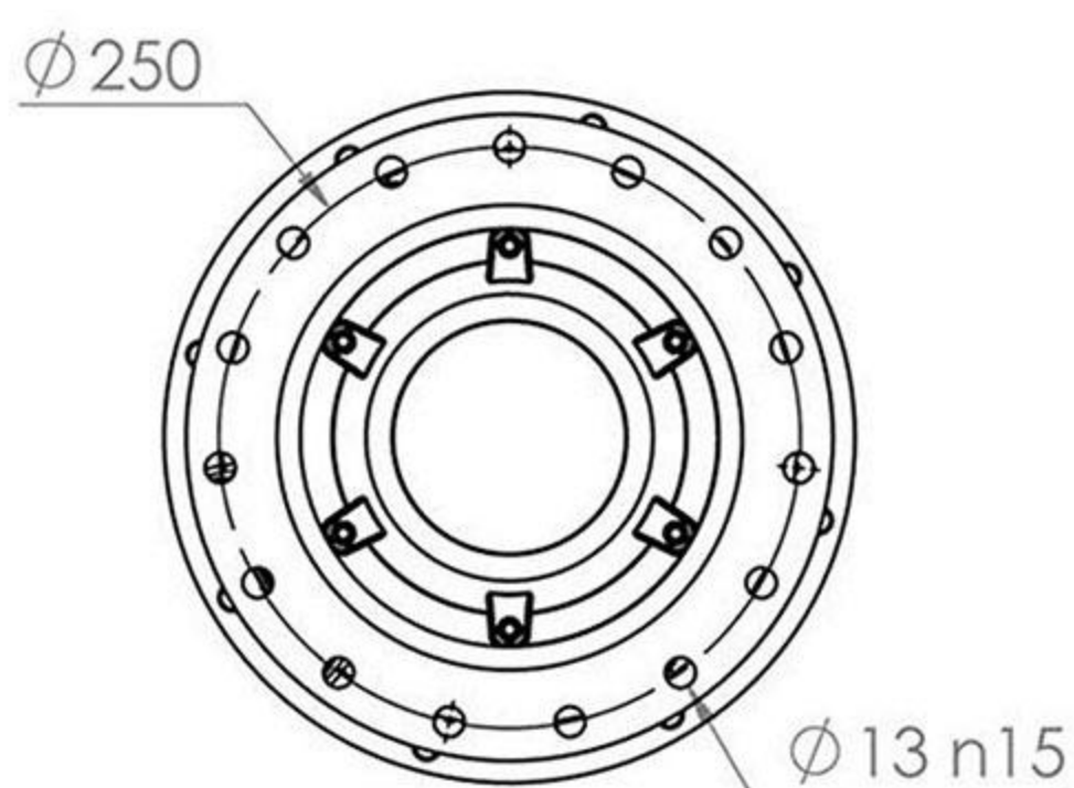
Output Flange Dimensions
