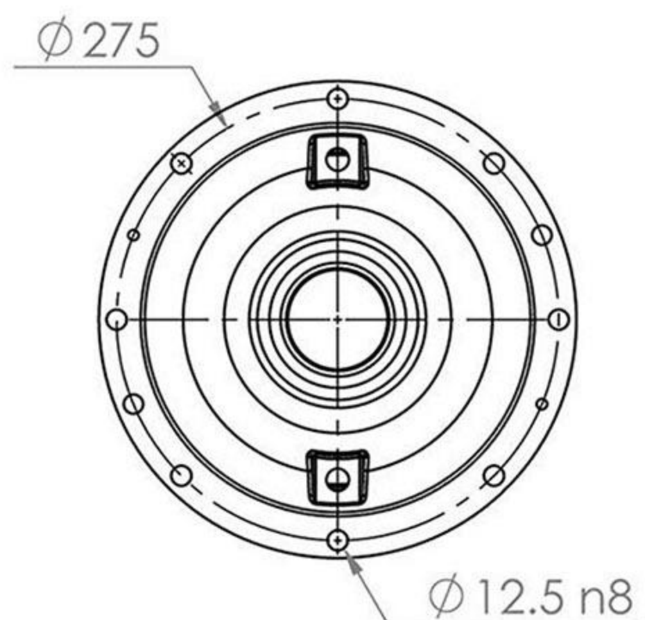
Output Flange Dimensions
